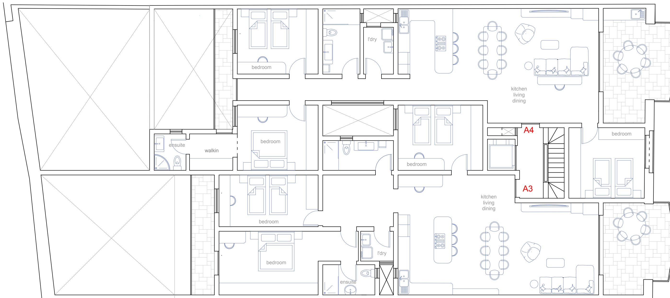
Proposed Second Floor
