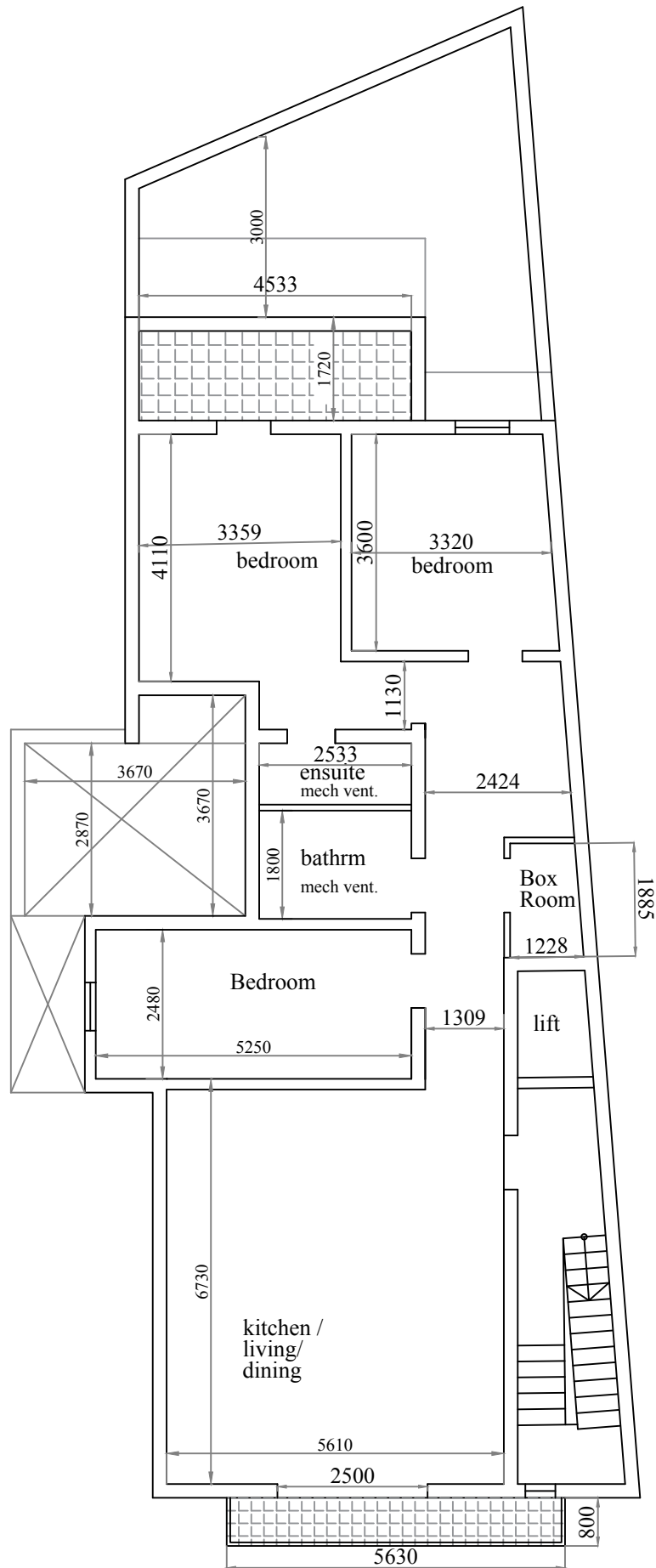
Proposed Third Floor Plan
